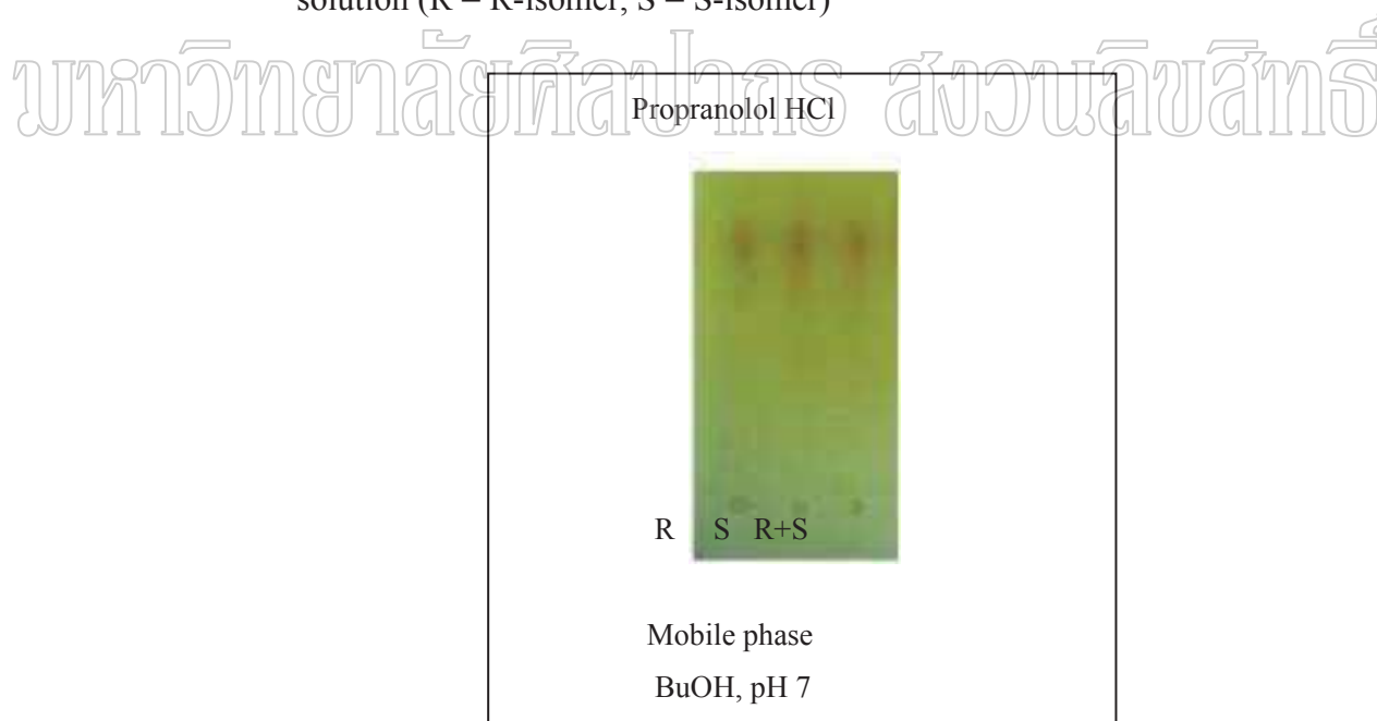
Figure 23 Photograph of the chromatogram racemic propranolol using the electrospun plate impregnated with L-mandelic. The same condition including developed distance : 4 cm, temperature: 22°C, detection: iodine solution (R = R-isomer, S = S-isomer)
