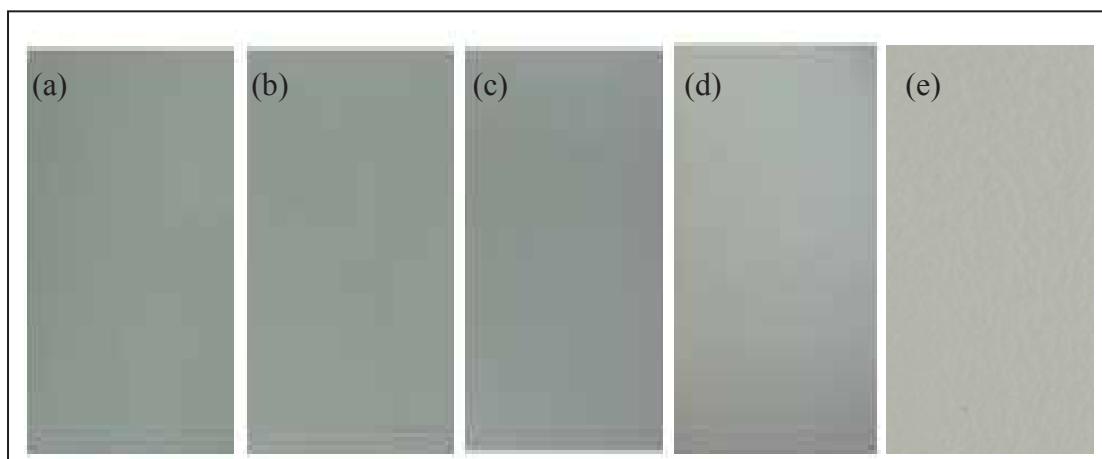
Figure 13 Appearance of plates including (a) electrospun plate from 2:1 ratio, (b) electrospun plate from 1:1 ratio, (c) electrospun plate from 1:2 ratio (d) silica commercial plate and (e) plate prepared by CA slurry spreading
