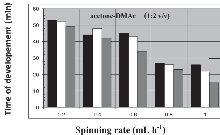
Figure 18 Dependence of the developing times on various spinning rates and Spinning times, Plate: electrospun mat from 17% w/v cellulose acetate in acetone-DMAC 1:2 v/v, spinning time : ■ = 2 h, □ = 4 h, ■ = 6 h
